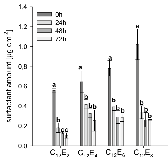
Fig. 7 Time-dependent changes in the amounts ( \mu\text{g cm}^{-2} ) of the monodisperse alcohol ethoxylates C_{12}E_2 , C_{12}E_4 , C_{12}E_6 and C_{12}E_8 remaining on Prunus leaf surfaces after spraying aqueous solutions of 0.1% leading to a surfactant coverage of 1 \mu\text{g cm}^{-2} . Amounts of the alcohol ethoxylates rapidly decreased within the first 24 h, whereas the rates of decrease levelled off between 24 and 72 h. Differential letters indicate significant differences between the different times at p < 0.05 . Bars represent means with standard deviations ( n = 4 )
