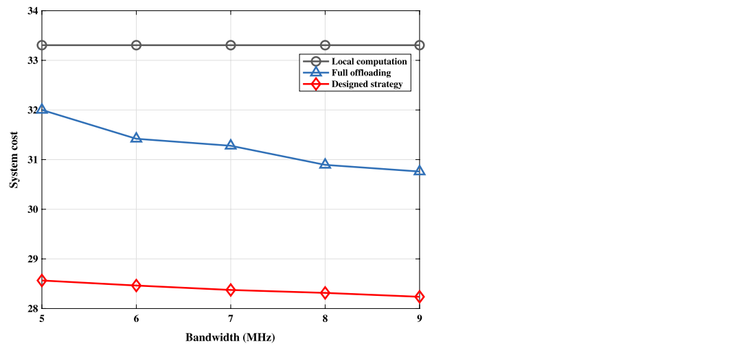
Fig. 6 System cost comparison of three schemes under the different values of bandwidth
