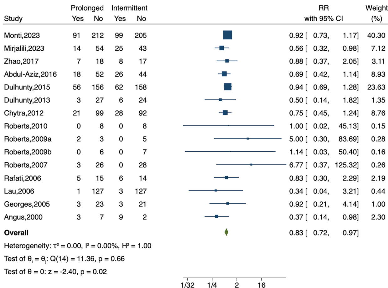
Random-effects DerSimonian-Laird model
