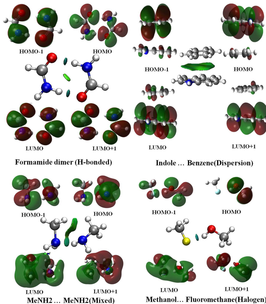
Fig. 3 The NCI plots and electron density of the frontier molecular orbitals (Carbon: grey, Nitrogen: blue, Oxygen: red, Hydrogen: white, Chlorine: yellow)
