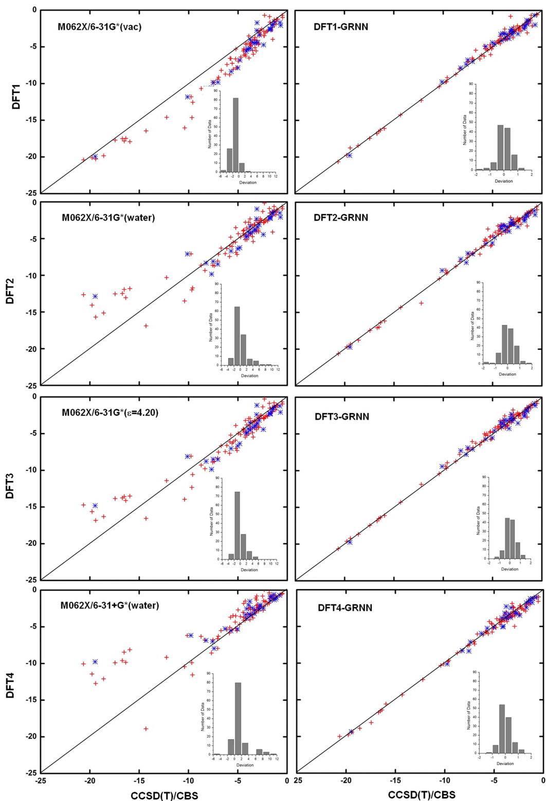
Fig. 4 NCIs calculated by DFT M06-2X (left) and DFT-GRNN (right) versus benchmark values. The insets are the deviation (calculated-benchmark) distribution relative to the benchmark values in each calculation (training set: red; test set: blue)
