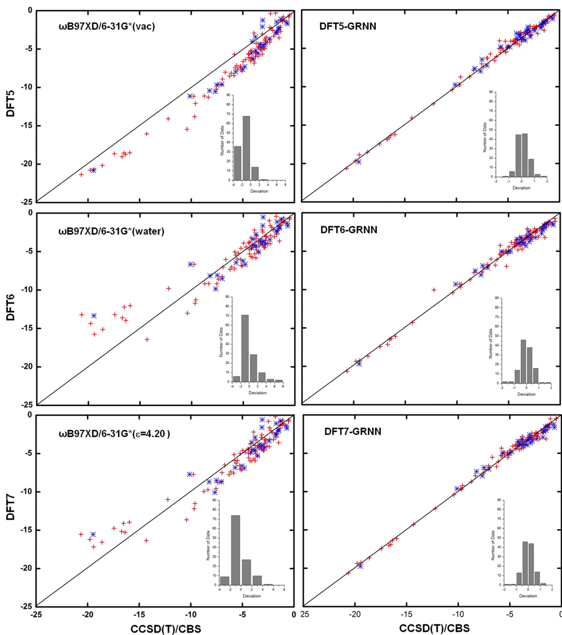
Fig. 5 NCIs calculated by DFT \omega B97XD and DFT-GRNN versus benchmark values. The insets are the deviation distribution relative to the benchmark values in each calculation (training set: red; test set: blue)
