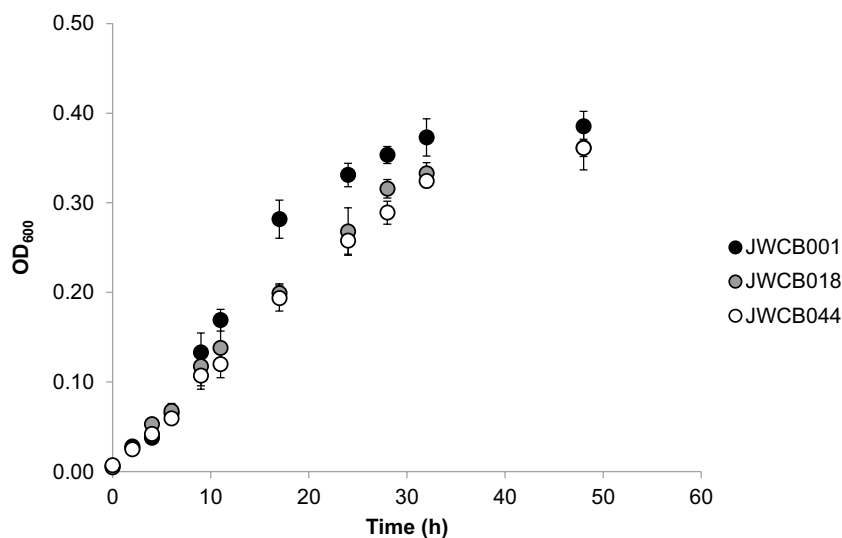
Figure 2 Growth profiles of C. bescii wild-type, JWCB018 and JWCB044 in LOD medium at 75°C.
