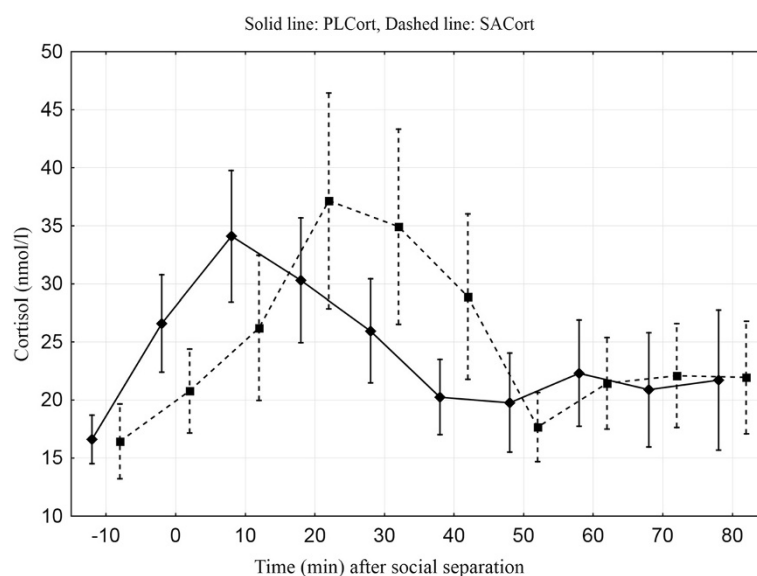
Figure 1 Plasma (PLCort) and salivary (SACort) cortisol concentrations (nmol/l) through a 90 min sequence with time zero allocated to the time of social separation. Values averaged across cow and calf subjects, given with standard errors. Time-series interpolated to 10 min equidistance with SACort concentrations multiplied by a factor of 10 for clarity. The series are slightly time-shifted to avoid overlapping error bars.
