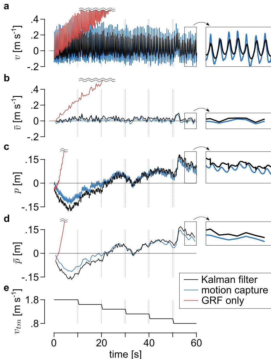
Fig. 3 Estimations of State Estimator and motion capture system. The plots show the subject's estimated a instantaneous speed v , b mean speed of each step, \bar{v} , c instantaneous position, p , and d mean position of each step, \bar{p} . All speeds and positions are in the lab reference frame. The values are estimated with the proposed Kalman filter (black line), motion capture system (blue line), and by simply integrating the ground reaction forces (red line). e The data are collected during a one-minute trial where the treadmill speed, v_{tm} , changes from 1.8 to 0.8 \text{m s}^{-1} as shown in the bottom plot. Panels at right provide an enlarged view of the final five seconds of data
