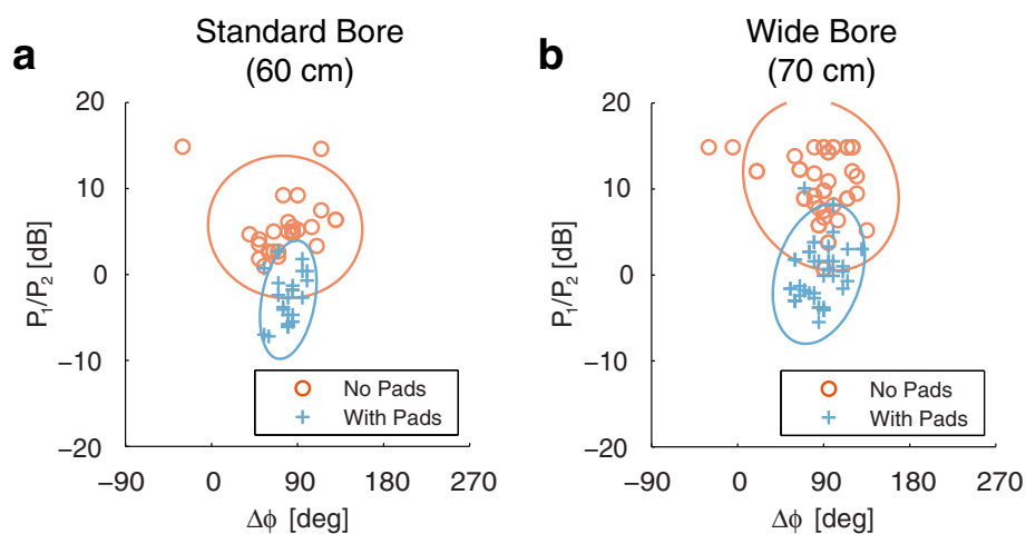
Fig. 3 Experimental RF shimming results acquired on the standard bore (a) and wide bore (b) system, together with corresponding 95 % confidence ellipses. RF-shim settings for images acquired in the long- and short-axis orientations were recorded separately
