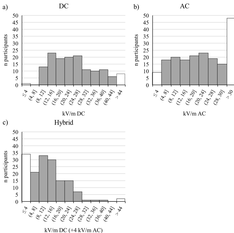
Fig. 6 Histograms of SIAM detection thresholds: For a DC EF, b AC EF, and c hybrid EF. In hybrid sessions, various DC EFs (x-axis) were always combined with an AC EF of 4 kV/m. White bars at the left and right edges reflect the participants with min or max termination criteria, where no detection threshold could be assessed
