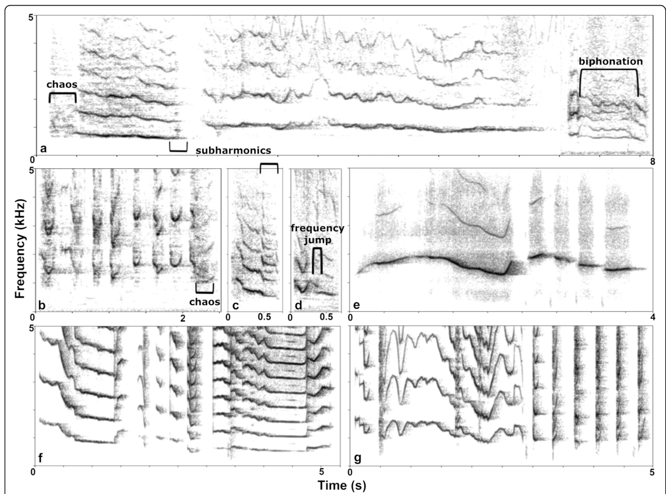
Fig. 5 Spectrograms: a–d Squeaks from four different adult female Asian elephants demonstrating intra-individual ( a + b ) and interindividual ( a–d ) variability in spectral and temporal features and containing examples of nonlinear phenomena: a long squeaks that were emitted as single calls and concatenated for display ( f , 55 years), b short squeaks that were emitted in a bout ( f , 23 years); c f , 60 years, d f , 48 years, e the first author whistling; f a balloon when letting the air stream through its tensed neck; and g the first author buzzing her lips
