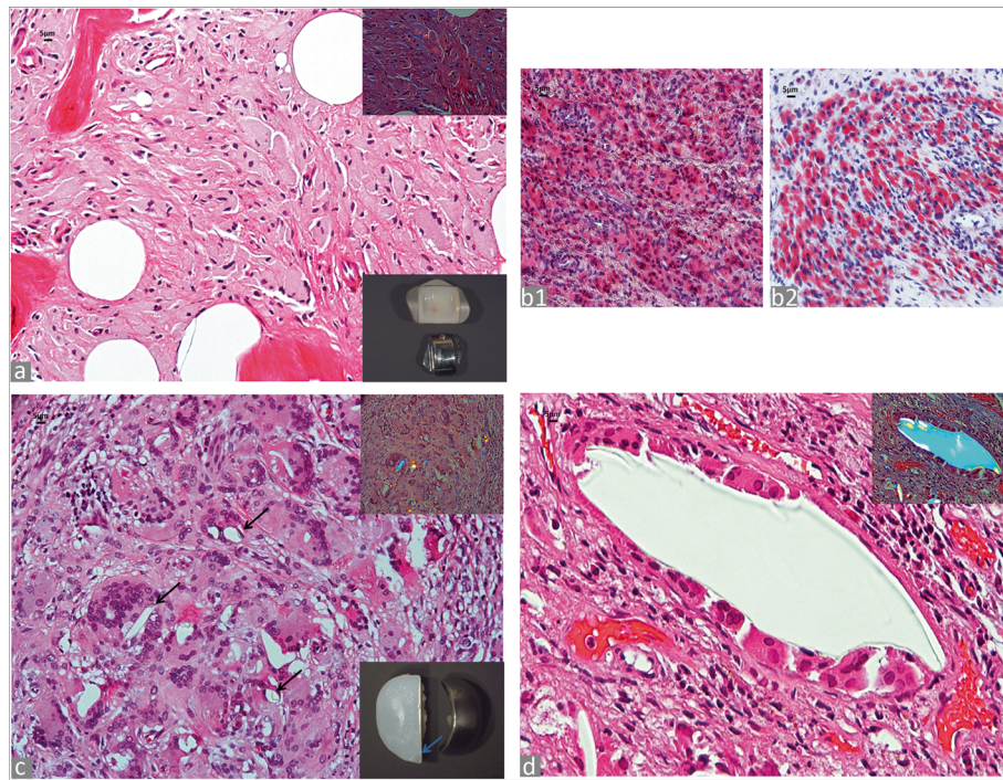
Fig. 3 Polyethylene (PE) particles. a Osteolysis with diffuse macrophage infiltrate containing PE micro-particles (H&E x 200), birefringent PE micro-particles under polarized light in the upper right inset (x 400), total ankle replacement implant in the lower right inset. b1 . Oil red O positivity for macrophage cytoplasm containing PE micro- and submicron particles in a MoP TKA implant (x 200); b2 . Oil red O positivity for macrophage cytoplasm containing tribocorrosion metallic particles in MoM HRA implant (x 200). c PE macroparticles (black arrows) in multinucleated giant cells (H&E x 200), birefringent particles under polarized light in the upper right inset (x 200), left unicompartmental knee implant with large area of PE abrasion/delamination (blue arrow) in the lower right inset. d PE supra-macroparticle lined by multinucleated giant cells in a case of failed total elbow prosthesis (H&E x 200), birefringent PE supra-macroparticle under polarized light in inset (x 200)
