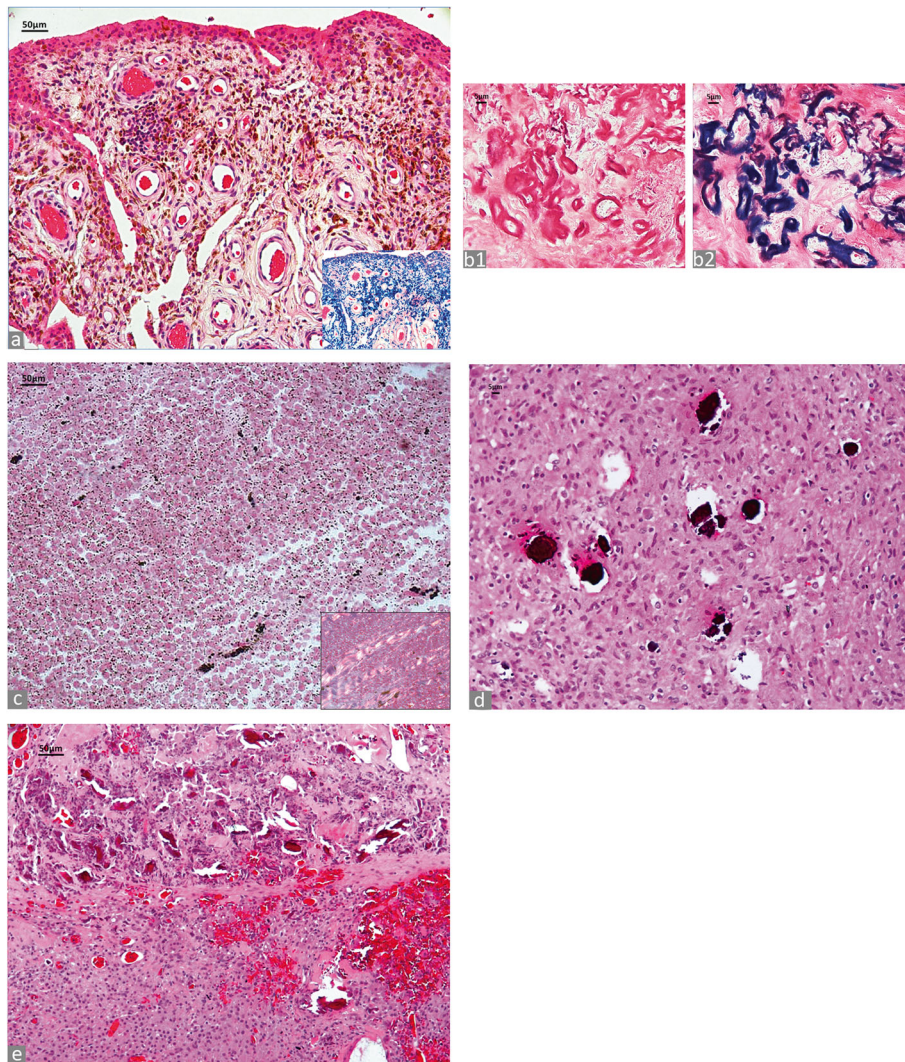
Fig. 7 Hemorrhage byproducts and calcific/osseous deposits. a Hemosiderin pigment in neo-synovium (H&E \times 100 ), hemosiderin deposits positive for PBR in inset (PBR \times 100 ). b1 Gama-Gandy bodies in failed MoP THA with hemorrhage secondary to multiple dislocations ( \times 400 ), b2 positivity to PBR reaction, PBR stain in inset ( \times 400 ). c Formalin pigment artifact, negative for PBR reaction (PBR stain \times 100 ) and with typical birefringence of the granules of formalin pigment under polarized light in inset ( \times 200 ). d Lime (dystrophic calcification) in periprosthetic neo-synovium of a case of hip implant failure (H&E \times 200 ). e Neo-synovium of a failed MoP THA implant for aseptic loosening/osteolysis with abundant osseous detritus embedded in the superficial layer (H&E \times 100 )
