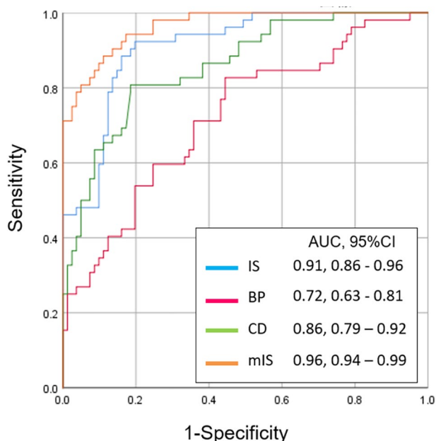
Fig. 3 Receiver operating characteristic (ROC) curve for the IS, BP, CD, and mIS methods. IS, Insall-Salvati (blue line); BP, Blackburne-Peel (red line); CD, Caton-Deschamps (green line); mIS, modified Insall-Salvati (orange line); AUC, area under the curve; CI, confidence interval
