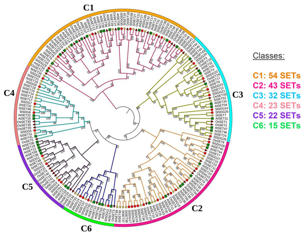
Fig. 3 Phylogeny of SET domain-containing genes of potato and Arabidopsis thaliana , Solanum lycopersicum , and Oryza sativa . We visualised the computed phylogenetic trees using iTOL [35]
