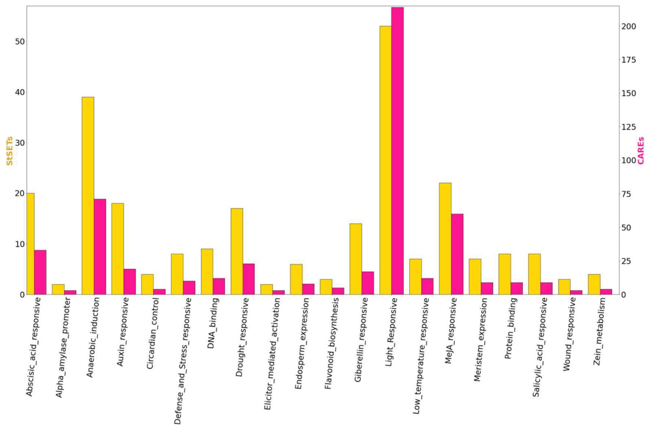
Fig. 4 The cis -elements (CAREs) with a frequency > 3 , detected within a 1 kb region upstream of the transcription start site. The yellow color bars indicate the number of genes in which respective cis -element is identified. The magenta color bars indicate the sum of respective cis -elements. We identified cis -elements within the promoter sequences using the PlantCARE database with a frequency cut-off of three for each cis -element [36]
