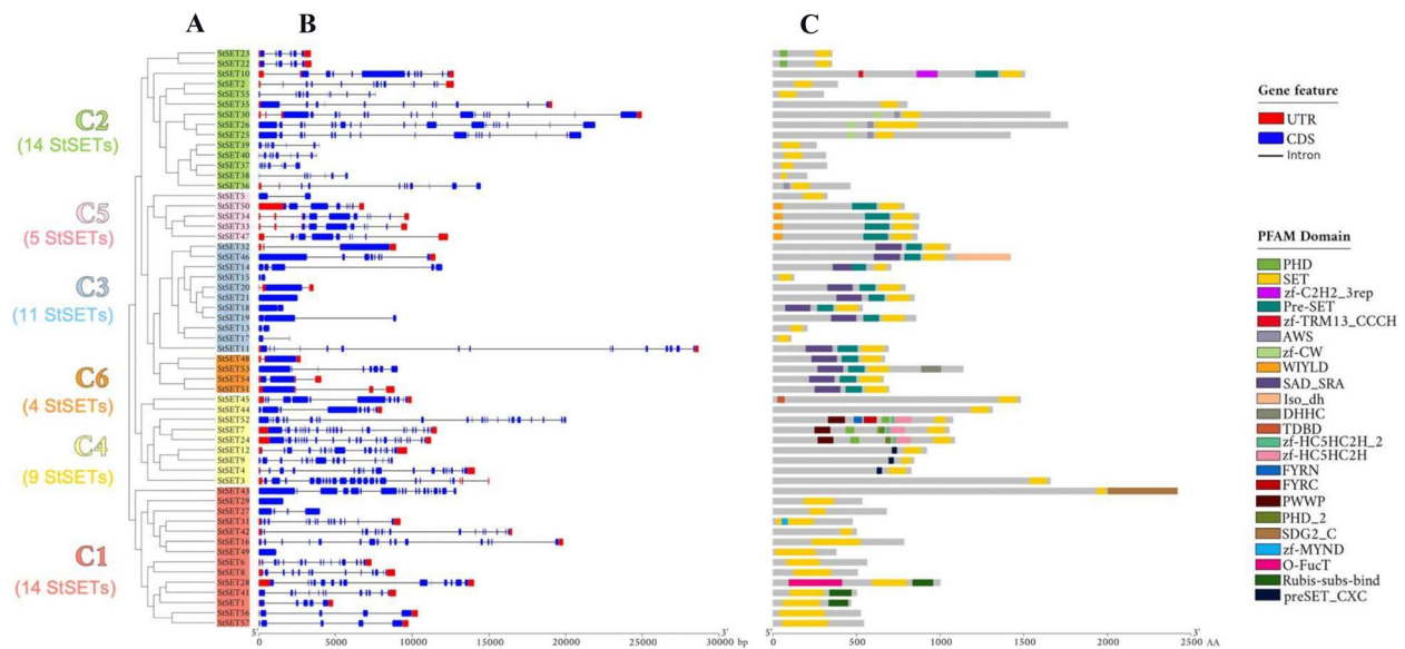
Fig. 2 Gene structure and protein domain organisation of StSET genes with respect to their phylogenetic order. A). The estimated phylogenetic tree for StSET genes, B). Gene structure of StSET genes, and C). Protein domain organisation of StSET proteins. We visualised the phylogenetic tree, the gene structure and the protein domain organisations using TBtools v1.098696 [34]
