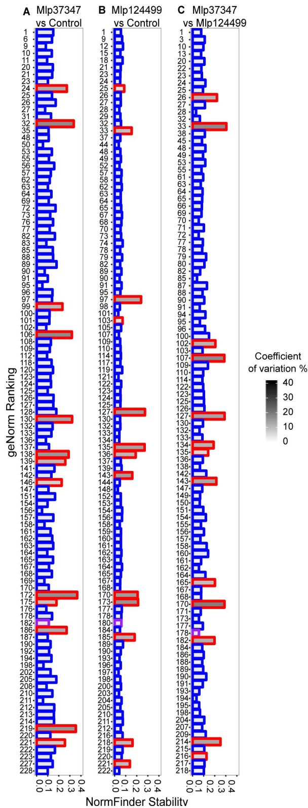
Fig. 4 Comparison of custom selected reference genes (blue border) and commonly used reference genes (red border) with geNorm ranking, NormFinder stability index and coefficient of variation for a Mlp37347 vs Control, b Mlp124499 vs Control and c Mlp124499 vs Mlp37347. The bar with purple border indicates the gene (NDUFA8) selected with the custom script that is also present in the common references
