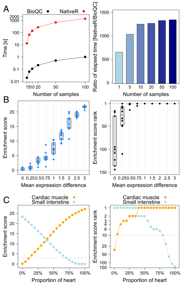
Fig. 1 Results of simulation studies a Speed benchmark. Left panel : running time of BioQC and R-native Wilcoxon test with simulated datasets of increasing sample sizes. Right panel : ratio of running time between the two implementations. b Sensitivity of BioQC revealed by simulations with model-generated data. Left panel : whisker-box-plot of BioQC enrichment scores of the selected gene set ( Y-axis ) against the average expression differences of genes in the set compared with genes not in the set ( X-axis ). Right panel : whisker-box-plot of ranks of enrichment scores. c Sensitivity of BioQC revealed by simulations with real-world data. Left panel : Enrichment scores of cardiac-muscle- and small-intestine-enriched genes as canine heart and jejunum samples are mixed with varying weights. Right panel : Ranks of enrichment scores plotted against varying weights
