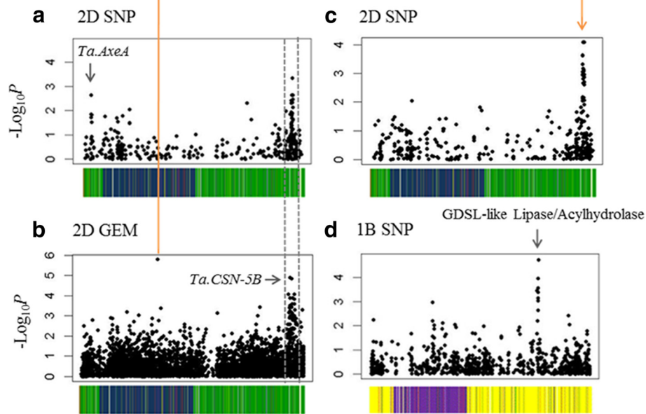
Fig. 3 Variation at both the sequence (SNP) and gene expression (GEM) level show high association with MOR. Two SNP association peaks for MOR were seen on chromosome 2D ( a ). The peak to the right of panel a was also identified in the GEM analysis ( b ). Several single GEM associations were also detected for MOR (see single GEM at the foot of the orange line in panel b as an example). Mapping transcript abundance (as RPKM) as a trait against the SNP data revealed the same 2D SNP peak for several single GEMs (see panel c for an example). A further SNP association for MOR was detected on chromosome 1B ( d ). The positions of candidate genes are indicated by arrows. -\text{Log}_{10}P values are plotted in wheat pseudomolecule order. Unigene order is colour-coded according to sequence similarity to B. distachyon chromosomes (blue = Bd1; yellow = Bd2; purple = Bd3; red = Bd4 and green = Bd5). Position of candidate genes are indicated by arrows
