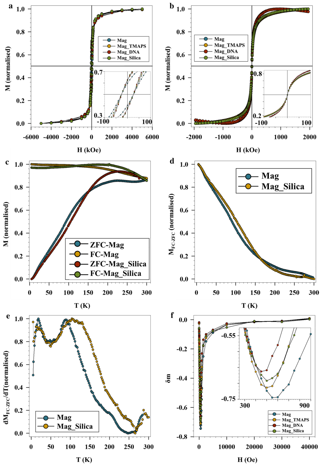
Fig. 4 Field dependence of magnetization for Mag, Mag_TMAPS, Mag_DNA and Mag_Silica at a 5 K and b 300 K. c ZFC-FC measurements, d M_{FC-ZFC} plots and e derivative of M_{FC-ZFC} plots for Mag and Mag_Silica. f \delta m plots at 5 K Mag and functionalized Mag samples
