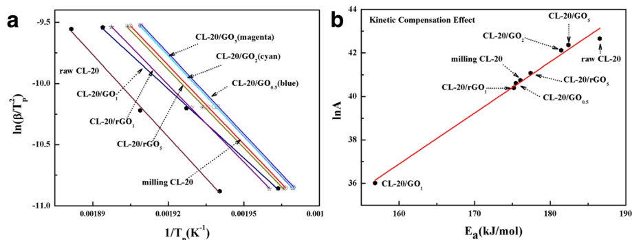
Fig. 5 a Kissinger plots of \ln(\beta/T_p^2) to 1/T_p . b Kinetic compensation effect for thermal decomposition of as-prepared samples
