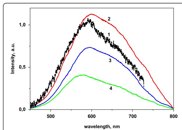
Fig. 5 Emission spectra of the \text{La}_{1-x}\text{Ca}_x\text{VO}_4 samples, \lambda_{\text{ex}} = 310 (1–3) and 290 nm (4); x = 0 (1), 0.2 (2), and 0.1 (3, 4), T = 77 K
