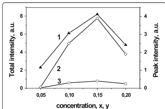
Fig. 9 Dependencies of the \text{La}_{1-x-y}\text{Eu}_y\text{Ca}_x\text{VO}_4 luminescence intensity on dopant concentration x, y ; total emission (1) and 622 nm peak intensity (2, 3); \lambda_{\text{exc}} = 405 (1, 2) and 473 nm (3)
