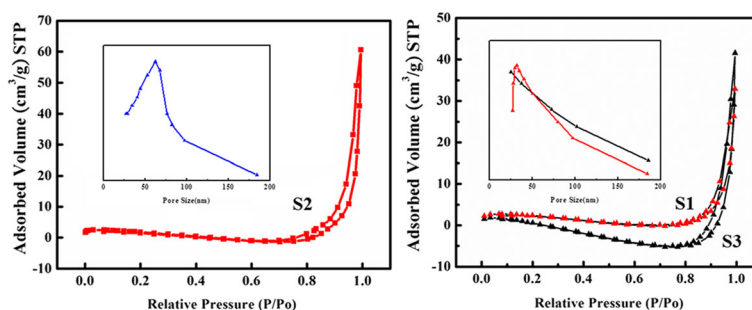
Fig. 6 N 2 adsorption-desorption isotherms for LiMn 2 O 4 nanofibers S2 (a), S1 and S3 (b), with insets showing the BJH pore size distributions for the corresponding samples
