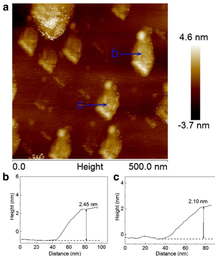
Fig. 6 a A typical AFM image of MoS 2 nanosheets obtained at 240 min and b, c the topographic height profiles of the two parts labeled in a
