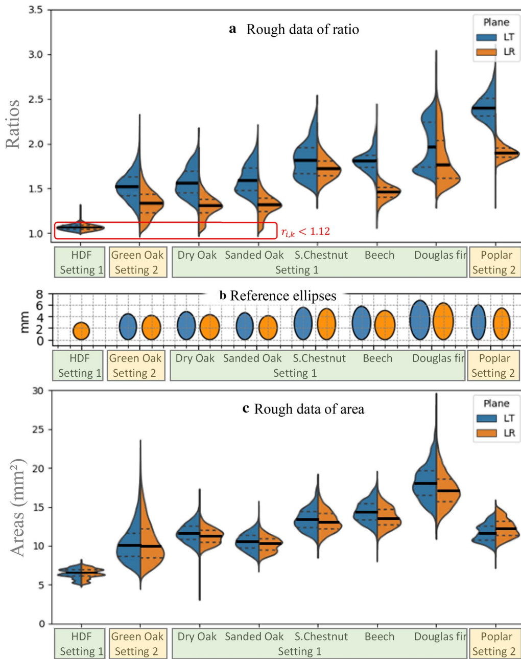
Fig. 7 Ellipse comparison between species: Ellipse RATIO by species displayed by violin plots (a): data from LT plane in blue, data from LR plane in orange (colors not relevant for HDF), medians (bolt lines) and 25th and 75th percentiles (dashed lines). Reference ellipse drawing from R_{ref} and S_{ref} , sorted as (a, b). Ellipse AREA data represented by species by means of violin plots, sorted as (a, c)
