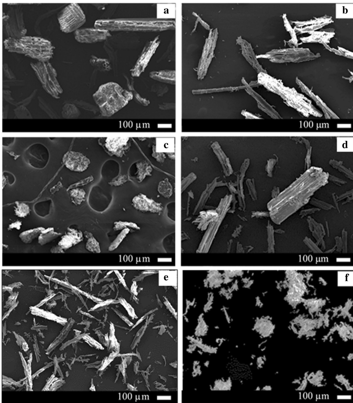
Fig. 4 The SEM image of WF. Heat drying condition: a 0 min, b 30 min and c 120 min of wet milling time. Freeze-drying condition: d 0 min, e 30 min and f 120 min of wet milling time
