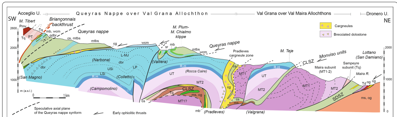
Fig. 5 Semi-schematic geological cross-section of the Maira-Sampeyre and Grana Allochthons and adjoining units. See Fig. 3 for location of the topographic line; the deepest parts of the section are projected from the SE over 1–5 km, complying with the thicknesses of the geological formations. The entire section has been affected by blueschist-facies metamorphism before its exhumation under greenschist-facies conditions. Stratigraphic abbreviations : L-MJ: Lower-Middle Jurassic coarse/chaotic carbonate breccias; LP: Lower Pliensbachian cherty marbles; LSI: Lower Sinemurian siliceous marbles; MT: Middle Triassic, with 1: Anisian-Ladinian evaporitic carbonates, and 2: Ladinian dolostones; Pmv: Permian meta-volcanics; PT: Permian–Triassic conglomerates (Verrucano Piemontese, “anagenites”); R-H: Rhaetian-Hettangian coral marbles; Tq: Lower Triassic (Werfenian) quartzites; USi: Upper Sinemurian turbiditic carbonate breccias and marbles; UT: Upper Triassic dolostones; Lithostratigraphic abbreviations : cg: cargneules (with dolostone/marbles blocks, particularly in the Pradleves cargneule zone); cs: calcschists; dbr: dolostone breccias; mb: metabasite; ms: mica-schist; mtbs: meta turbiditic black shales; og: orthogneiss; qdbr: quartzite and dolostone breccias (Longet breccias, LB in Fig. 3); sr: serpentinite; wcm: whitish cherty marbles
