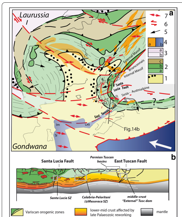
Fig. 14 Interpretative configuration of the post-Variscan setting (at c. 270 Ma) based on a modified version of Fig. 2 in Matte (2001). The scheme shows a possible frame of the Variscan belt of western Europe and north Africa, with the main Upper Carboniferous-Permian regional fault systems and related continental basins (after Burg et al. 1994). The original scheme of Matte (2001) is modified taking into account the data and interpretations proposed in this work. The Santa Lucia Fault (whose remnants are documented in the lower to mid-crust shear zone in the Alpine Santa Lucia Nappe), and the East Tuscan Fault (remnants in subsurface of Pontremoli and Larderello deep well) in the Apennines are represented. The East Tuscan Fault is prolonged southwards into the Lagonegro-Imerese-Sicani marine rifted domains (Catalano et al. 1995) westernmost extension of the Permian rifted basin related with Neo-Tethys (Ziegler and Stampfli 2001; Stampfli et al. 2002; Garfunkel 2004; Xyapolis et al. 2006; Schettino and Turco 2011). (1) Gondwana and Gondwana-derived crust blocks (Apulia and Adria figured); (2) Southern Europe Variscan belt: (a) low-grade external and nappe zone dots foreland domains, (b) axial zone medium to high grade units, suture/s and Ordovician arcs, (c) hinterland and Variscan retrowedge (Armorica, Hun or Brunia terranes); (3) (a) Laurussia-derived blocks of the northern continent; (b) inner domains of the South Europe Variscan orogen; (4) Permian sedimentary basins: (a) continental, (b) marine; (5); main vergence of the nappes; (6) kinematics of late Palaeozoic regional faults; (7) extension direction during Upper Carboniferous-Permian. The possible positions of the Briançonnais, South-Alpine and Austro-Alpine domains are also reported (see also Festa et al. 2018; Balleve et al. 2018 and references); thin dashed red lines represent dyke trend in Calabria (after Festa et al. 2010). Si: Sicani; Im: Imerese; Lag: Lagonegro; Ca: Calabria; Tu: Tuscany; Car: Carnia; IV Ivrea Zone; EL: External Ligurian; Z: Zicavo Shear Zone; P: Posada-Asinara; G: Grighini Shear Zone. (b) Conceptual schematic cross-section to envisaged the proposed tectonic scenario for late Palaeozoic in Central Mediterranean. The regional cross-section is traced not-perpendicular to the main regional fault systems to show and insert all the late Palaeozoic crustal domains and the different zones of South Europe Variscan orogen discussed in the text
