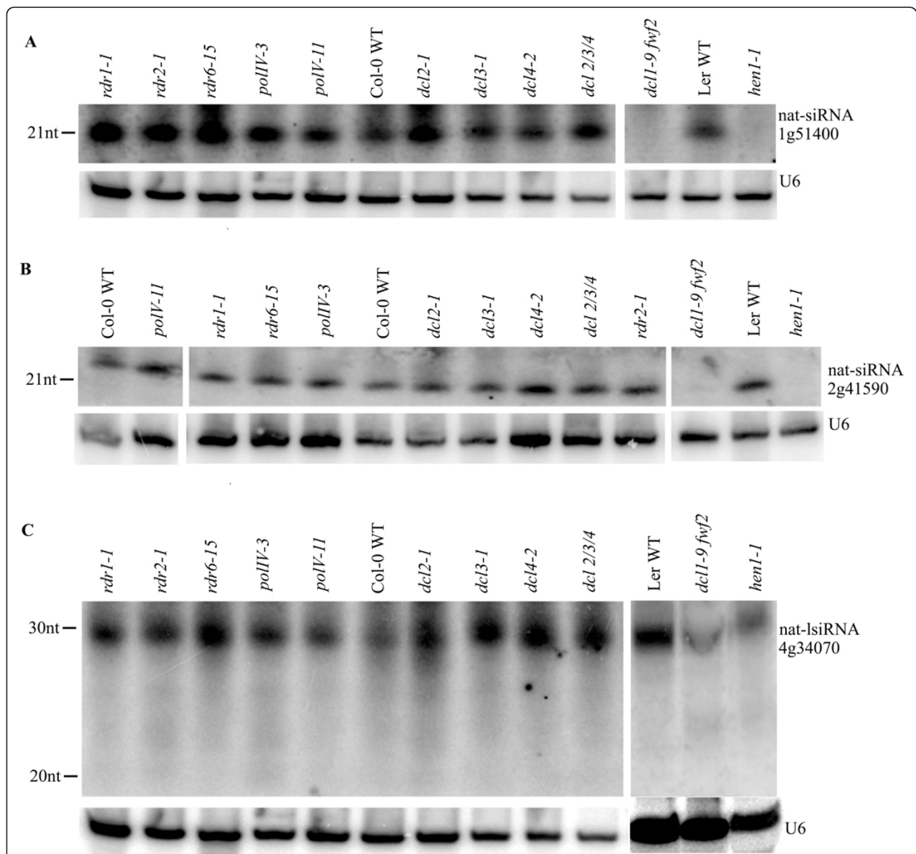
Figure 4 Biogenesis of nat-siRNAs that depend on DCL1. (a-c) Accumulation of nat-siRNA1g51400 (a), nat-siRNA2g41590 (b) and nat-siRNA4g34070 (c) is shown in various dcl , rdr , polIV and polIV mutants. Total RNA (75 to 100 µg) was used for Northern blot analysis. LNA probes complementary to each nat-siRNA were used. U6 was an internal control to show equal loading. The same results were obtained from two biological replicates.
