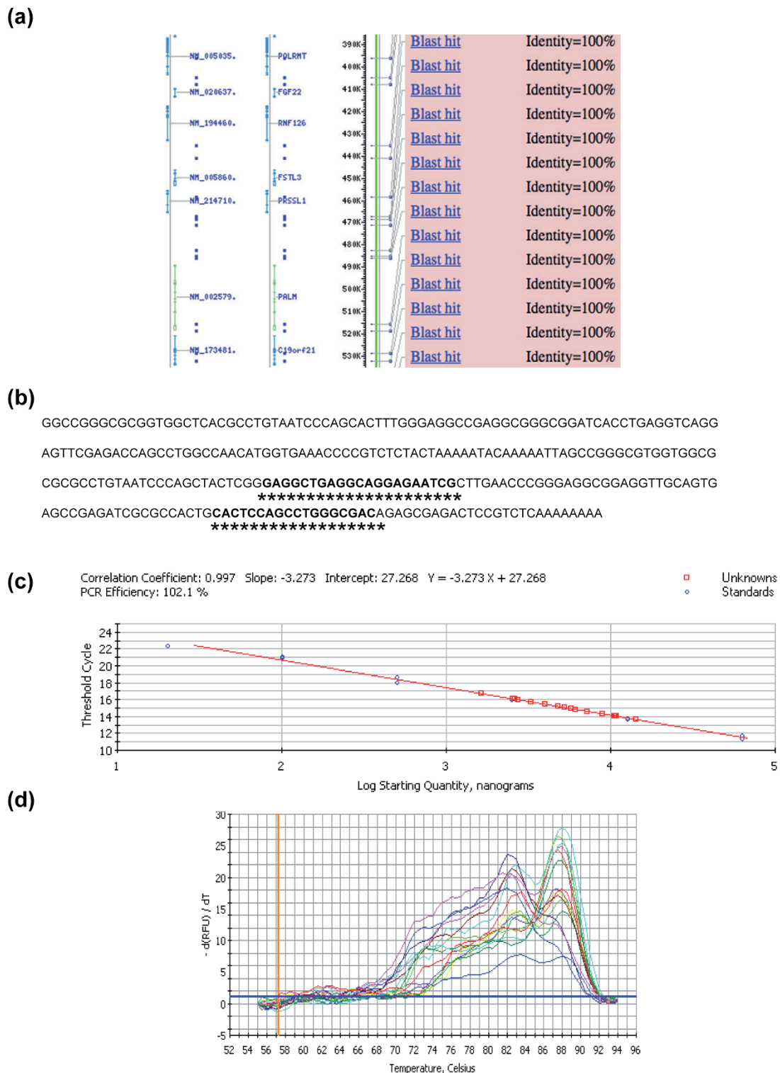
Figure 2 EAR amplification protocol in RNA from total blood. (a) BLAST analysis for Alu repeat distribution in the human genome. Alu repeat sequences are present in the UTRs of many genes. The small blue points indicate the homologous sequences at the Alu human consensus repeat. (b) Alu human interspersed repetitive sequence and primers used in this study for EAR amplification. (c) C_q of EAR mRNA plotted against the log of the relative initial amount of the pooled cDNA. (d) Melt-curve diagram generated from the amplification as described in (c).
