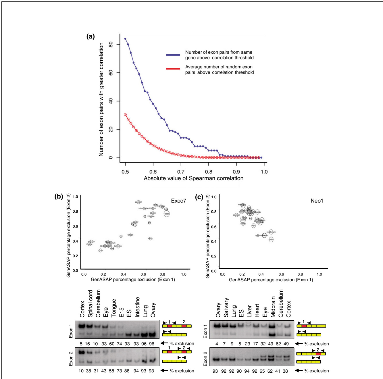
Figure 2 Coordination between AS events belonging to the same genes. (a) The correlation between the alternative splicing (AS) levels of pairs of alternative exons belonging to the same genes was assessed using standard Spearman correlation. The cumulative distribution plot shows the number of exon pairs (y-axis) observed to have an absolute value standard Spearman correlation higher than the value given on the x-axis. The blue curve with closed circles represents the number of observed exon pairs from the same gene above a given correlation threshold. The red curve with open circles is the average number of random pairs above a given correlation threshold, as determined using permutation resampling analysis (see Additional data file 1 [Materials and methods]). Also, representative examples of pairs of alternative exons with correlated splicing levels are shown (b) for a pair of exons with positively correlating inclusion levels from the Exo70 gene and (c) for a pair of exons with negatively correlating inclusion levels from the Neo1 gene. Upper panels show plots comparing the GenASAP percentage exon exclusion levels for each exon in a correlating pair, with the percentage exclusion levels for each exon separately plotted on the y-axis and x-axis. Circle sizes indicate relative transcript levels for the corresponding gene in each tissue shown, with larger circles indicating higher transcript levels. Lower panels show radioactive reverse transcription polymerase chain reaction (RT-PCR) assays performed with primer pairs targeted to constitutive exons flanking each alternative exon in a correlated pair. Percentage exclusion levels for each alternative exon, as measured using a phosphorimager (see Materials and methods), are shown. Additional examples of correlated pairs of exons validated by RT-PCR assays are shown in Additional data file 1 [Figure 2]. ES, embryonic stem cells.
