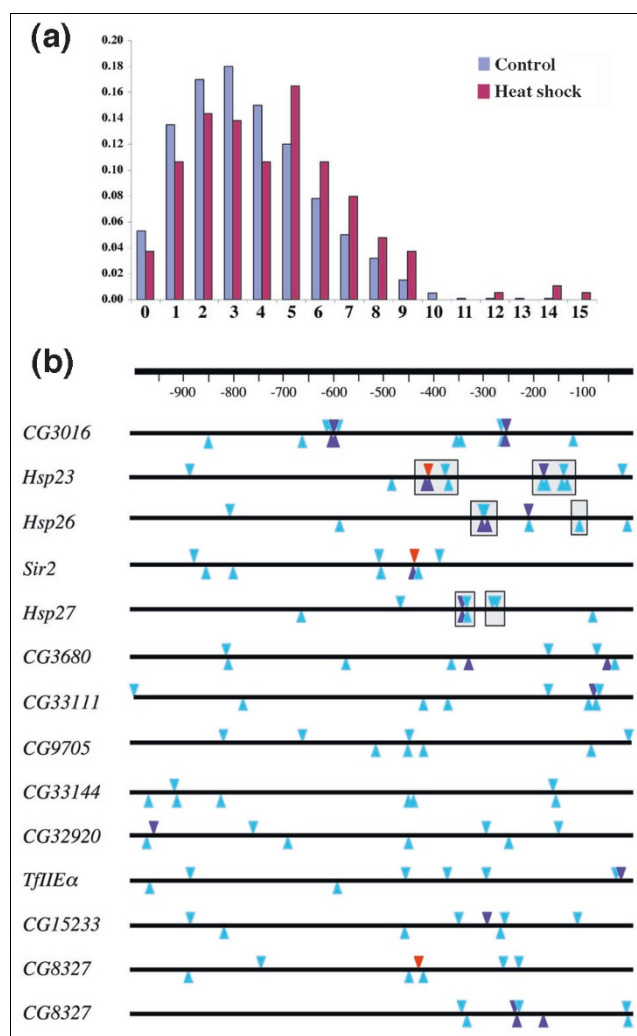
Figure 7 Predicted Hsf-binding sequences in the 1-kb region upstream of Hsf-binding genes. (a) Plot of the distribution of the number of predicted sites as a proportion of the population of anti-Hsf-enriched (Heat shock) or non-enriched (Control). (b) The relative position of predicted Hsf sites for each of the genes containing eight or more sites. The annotated gene start is on the right. Red triangles, perfect match; purple, one mismatch; light blue, two mismatches. Gray boxes represent the known HSEs upstream of Hsp23 , Hsp26 and Hsp27 .
