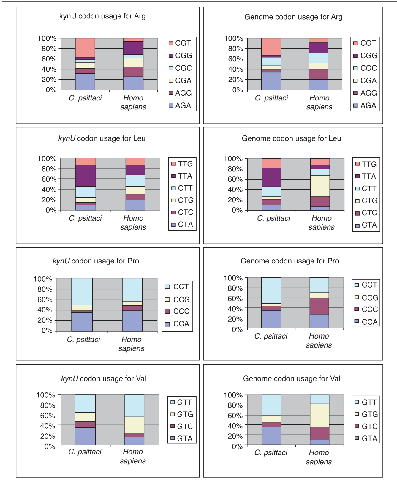
Figure 3 Comparison of codon usage (arginine, leucine, proline and valine) for kynU genes from C. psittaci and H. sapiens with the corresponding whole-genome codon usages.
