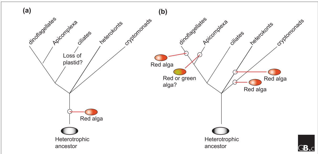
Figure 1 Schemes outlining two competing hypotheses for plastid origin(s) in algae containing secondary red algal symbionts. (a) New data from nucleus-encoded genes whose products are targeted to the plastid, and new data on dinoflagellate and Perkinsus plastids suggest that one secondary endosymbiotic origin spawned multiple groups, whereas (b) the canonical interpretation is that all these groups arose through independent secondary endosymbiotic events. Secondary endosymbioses are represented as introgressions of the red alga (or perhaps a green alga in the case of Apicomplexa) into circles within the lines of vertical descent. If scenario (a) is correct, ciliates have lost plastids secondarily, as have subgroups within the other lineages.
