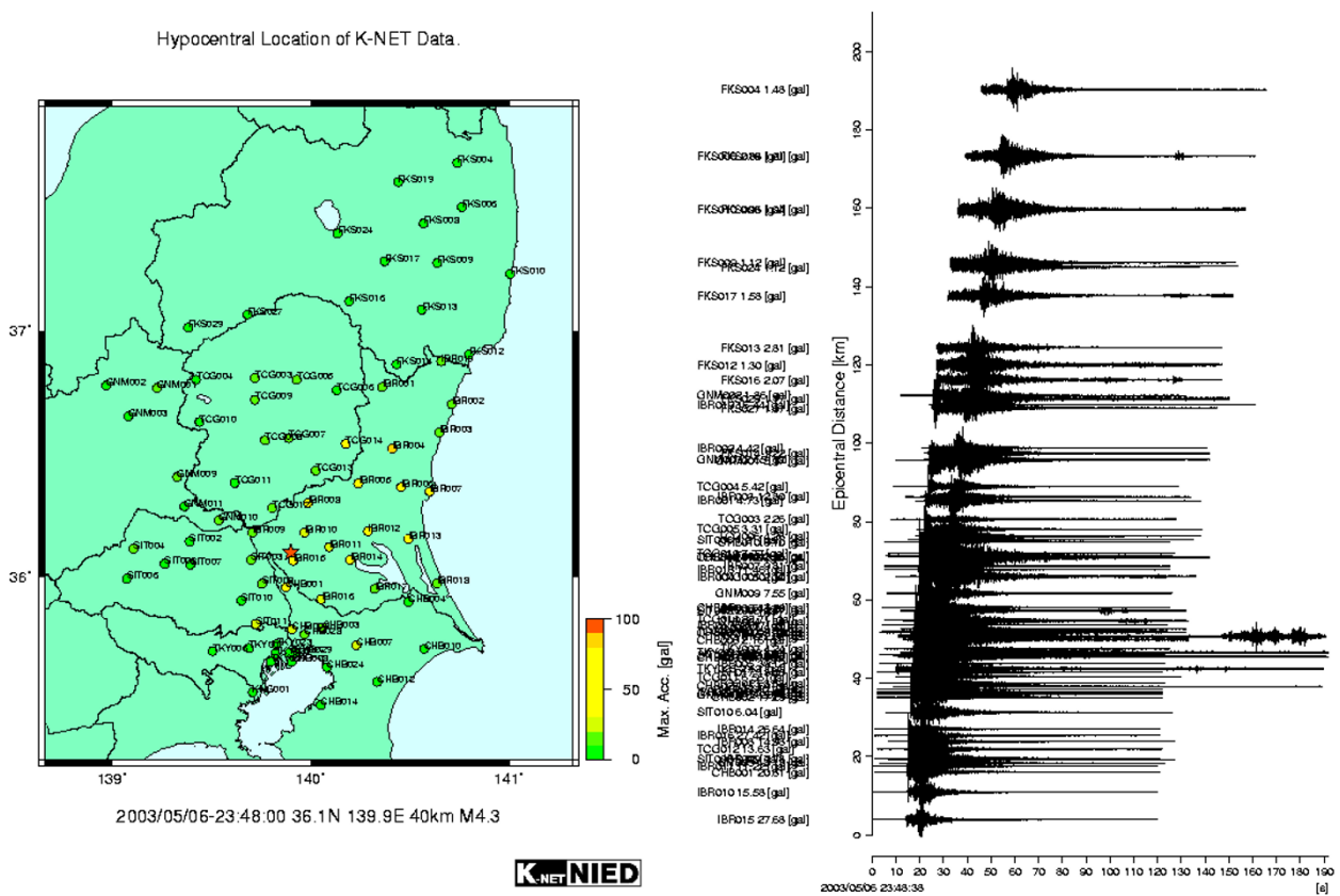
Fig. 14. An example of web screen image of the acceleration map and the paste up of strong motion records associated to a moderate earthquake in southwestern Ibaraki Pref. 1 gal corresponds to 1 m/s/s.
