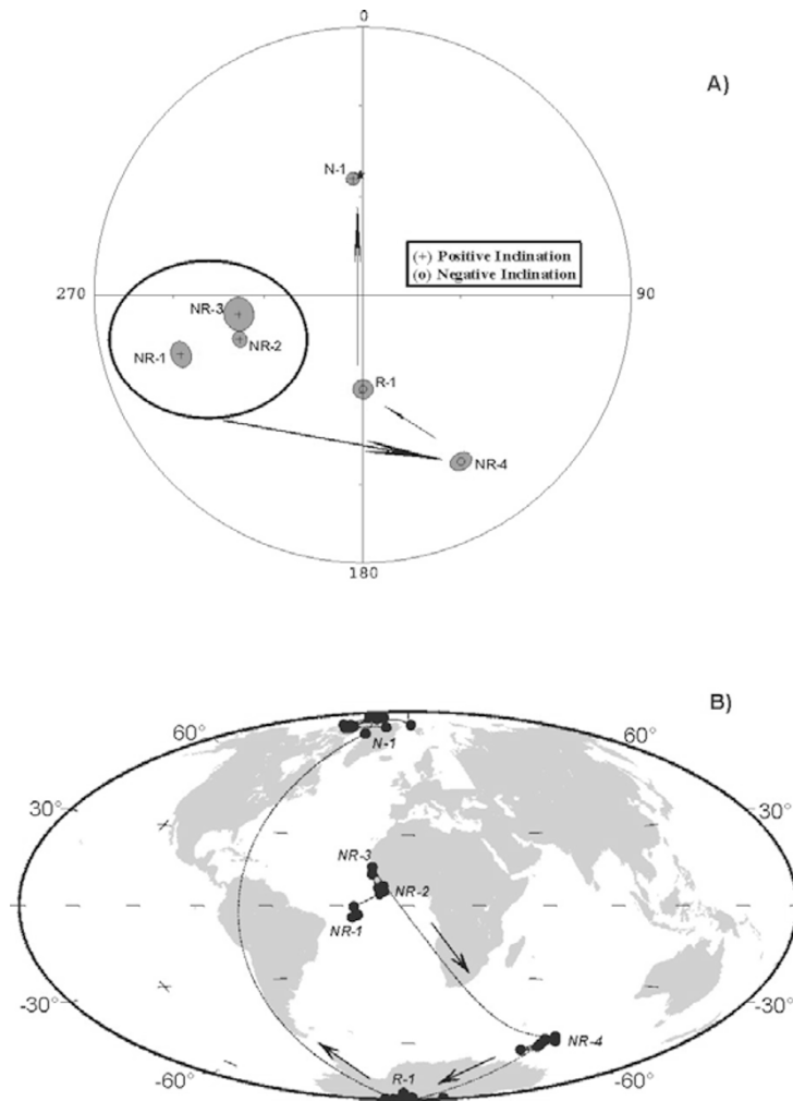
Fig. 7. (a) Equal area projections of the flow mean characteristic paleodirections of Akhalkalaki volcanics. Circles/crosses denote the negative/positive inclination, respectively. (b) The path of the virtual geomagnetic pole positions.
