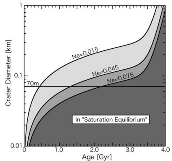
Fig. 6. Relationship between age and maximum size of saturated craters for each equilibrium level. The maximum size of saturated craters is obtained by calculating a node between the SFD of a saturated crater (Eq. (3)) and the ideal SFD expected for a given age. The ideal SFD can also be calculated from the cratering chronology (Eq. (2)) and the population SFD.
