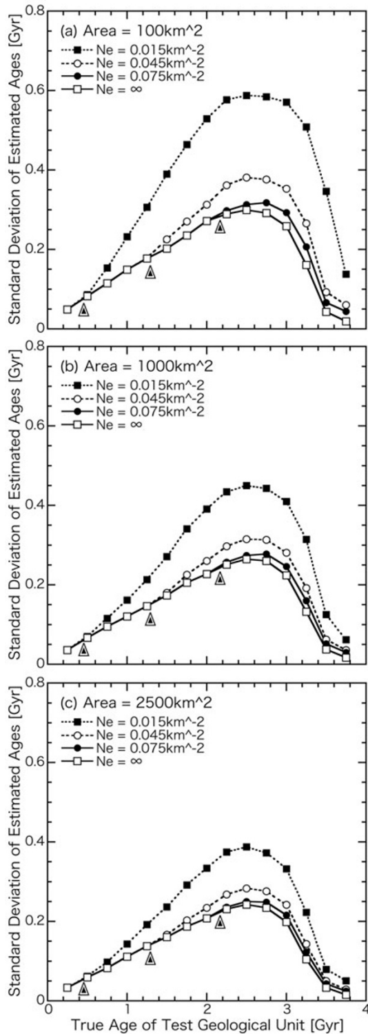
Fig. 5. Standard deviation of estimated ages as a function of the true age of the test geological unit. Triangle indicates the age when a 70 m-diameter crater is saturated for a given equilibrium level (see Fig. 6).
