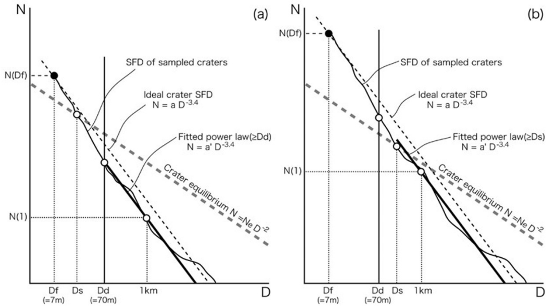
Fig. 1. Schematic representation of crater SFD measurement. Relative age is obtained by fitting the population SFD, N(D) = \alpha D^{-3.4} to SFD of craters \geq D_m . (a) D_d \geq D_s . Craters \geq D_d are used for SFD measurement (i.e., D_m = D_d ). (b) D_d < D_s . We use D_m = D_s .
