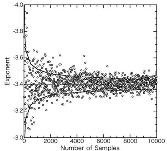
Fig. 2. Exponent of the power-law fitted to SFD for the sampled crater set as a function of the number of samples. The exponent assigned to the crater population SFD is -3.4 . Solid lines denote one standard deviation.
