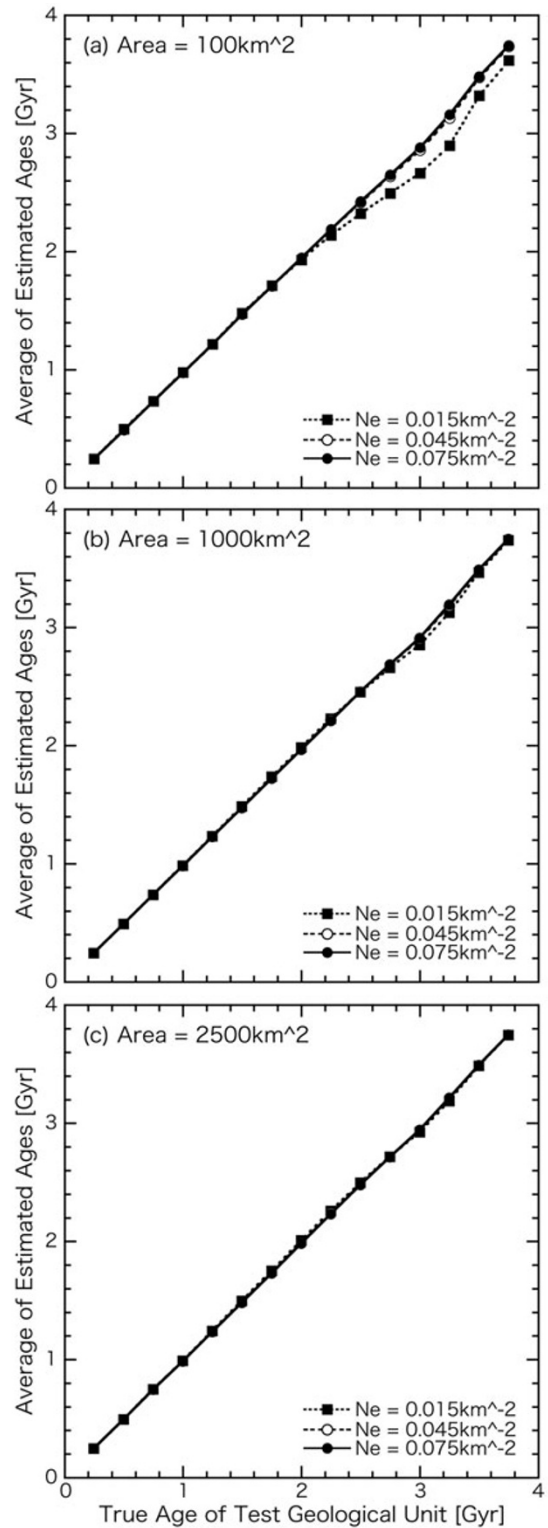
Fig. 4. Comparison of the average of estimated ages and the true age of the test geological unit for 100, 1000, and 2500 \text{ km}^2 .
