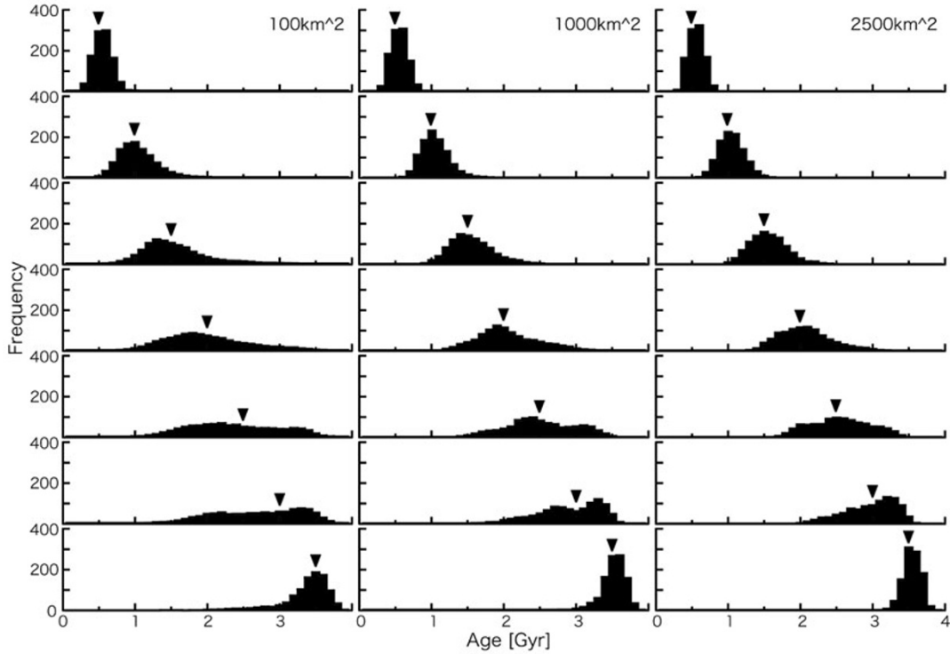
Fig. 3. Histogram of estimated ages for N_e = 0.015 . Filled inverse triangle indicates the true age of the test geological unit.
