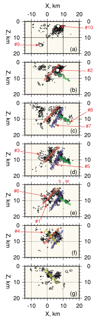
Fig. 5. Depth distribution of the relocated hypocenters on the X-Z cross-sections at (a) Y = 16 km, (b) Y = 12 km, (c) Y = 8 km, (d) Y = 4 km, (e) Y = 0 km, (f) Y = -4 km and (g) Y = -8 km. In these cross-sections, events located in the range \pm 2 km from the planes were plotted. The translucent red, blue and green thick lines indicate the estimated fault planes. The symbols S and M at the top of (e) indicate the locations of the Suwatoge Flexure and the Muikamachi Faults, respectively. The open circles with the numbers are the major events listed in Table 1.
