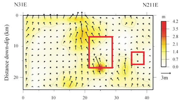
Fig. 2. Source model composed of two asperities. The model is superimposed the inverted slip contours by Honda et al. (2005).
