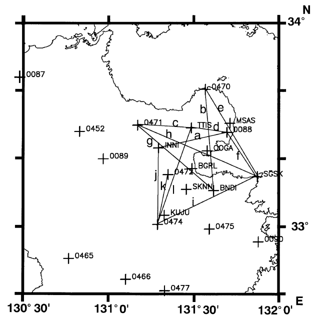
Fig. 2. GPS sites employed in this study. Lower case letters (a-l) show the baselines of which change rates are shown in Fig. 3.
