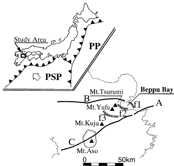
Fig. 1. Location map of the study area. PP: Pacific Plate, PSP: Philippine Sea Plate, A: Median Tectonic Line (MTL), B: Kurume-Hiji Line (KHL), C: Oita-Kumamoto Tectonic Line (OKTL), f1: Beppu Bay Cross Fault (BB), f2: Asamigawa Fault (AsF), f3: Tsuzura-Shonai Fault (TSF). (Modified from Sasada 1984 and NEDO, 1990).
