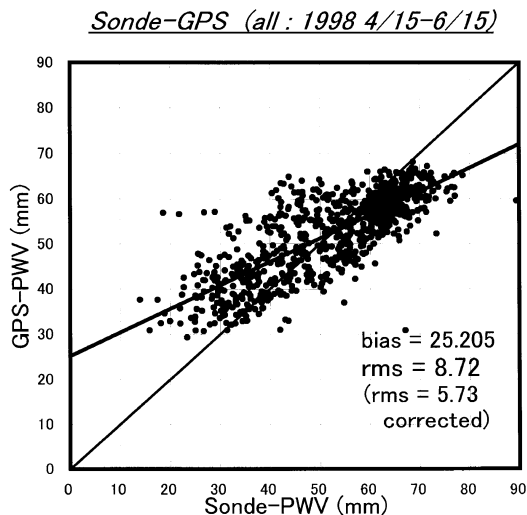
Fig. 3. GPS-PWV vs. Sonde-PWV. A linear regression line (thick line) is drawn using the least-squares method. Thin line is y = x .
