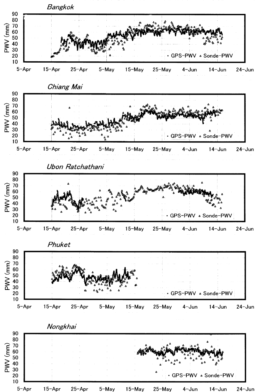
Fig. 2. Time series of GPS-PWV (black circle) and Sonde-PWV (white triangle) from April 15 to June 15, 1998.
