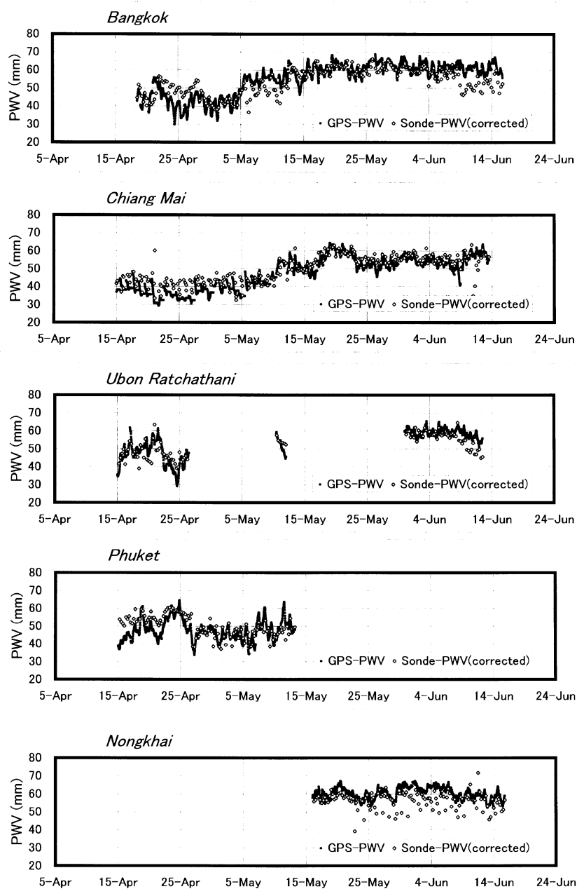
Fig. 4. Time series of GPS-PWV (black circle) and Sonde-PWV (white diamond) after correction by linear regression analysis. Bad sonde data with greater than 2.5 sigma RMS were also discarded.
