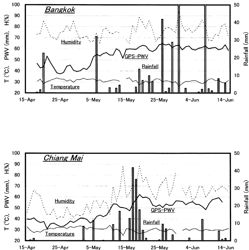
Fig. 5. Daily mean time series of GPS-PWV (thick lines), Temperature (thin lines), Humidity (dots) and Rainfall (bars) from April 15 to June 15, 1998.
