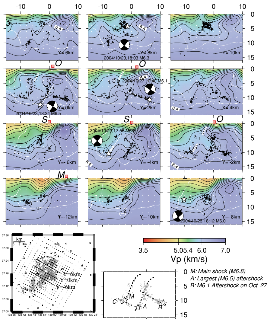
Fig. 3. Across-fault vertical cross sections of P -wave velocity. Small black and white crosses show hypocenters of aftershocks and grids, respectively. DWS values are greater within the area shown by white broken lines. Large stars and small black crosses denotes hypocenters of the main shock, aftershocks whose magnitude is greater than or equal to 6.0 and other aftershocks (27 Oct. 2004–21 Nov. 2004), respectively. Moment tensor solutions by the F-net, NIED are also shown by lower hemisphere projection on the section. Thin white broken lines from stars show plausible fault planes of the main shock, the largest aftershock and the M6 aftershock on Oct. 27. Thick white broken lines show large slip areas (asperities) of the main shock by (Yagi, 2005). Red boxes show surface traces of major active faults (M: Muikamachi, S: Suwatoge, O: Obiro). Right-bottom figure shows schematic presentation of some major aftershock alignments (see text for details).
