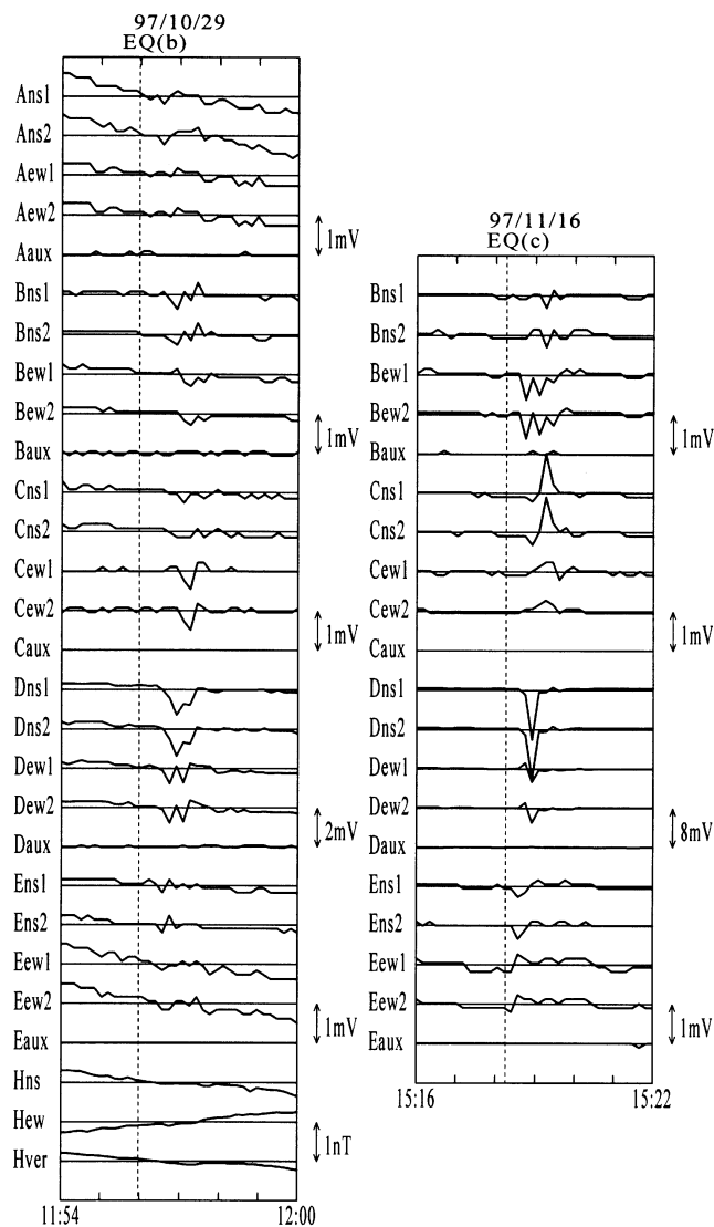
Fig. 8. Electric field changes (mV/100 m) at each site for 3 minutes before and after the co-seismic change associated with b and c earthquakes (see Table 1). Measurement interruption: line of Caux (97/10/29), site A and line Caux (97/11/16).
