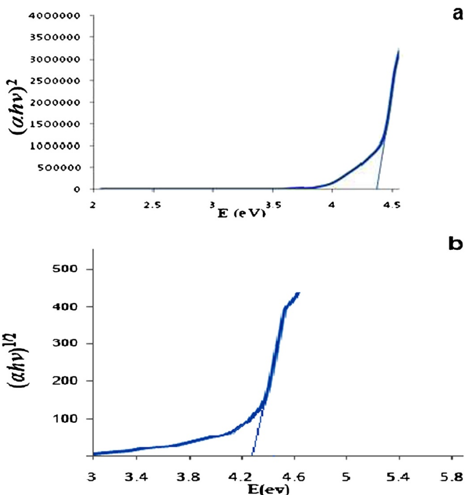
Figure 6 Direct and indirect allowed energy gap for P V. (a) Direct allowed energy gap for P V (\alpha h\nu)^2 . (b) Indirect allowed energy gap for P V (\alpha h\nu)^{1/2} .
