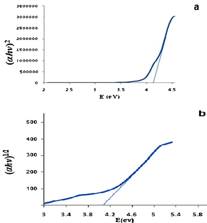
Figure 3 Direct and indirect allowed energy gap for P II. (a) Direct allowed energy gap for P II (ahv)^2 . (b) Indirect allowed energy gap for P II (ahv)^{1/2} .
