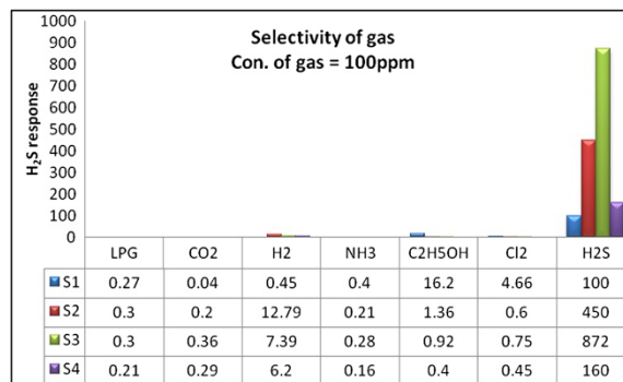
Figure 9 Selectivity of nanostructured CuO thin films for different gases.
