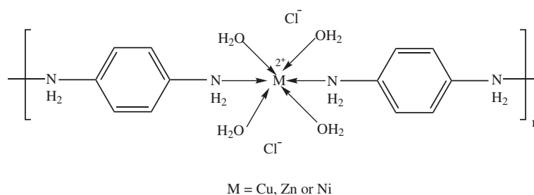
Scheme 1 One-dimensional linear coordination polymers comprising a repeat unit.
