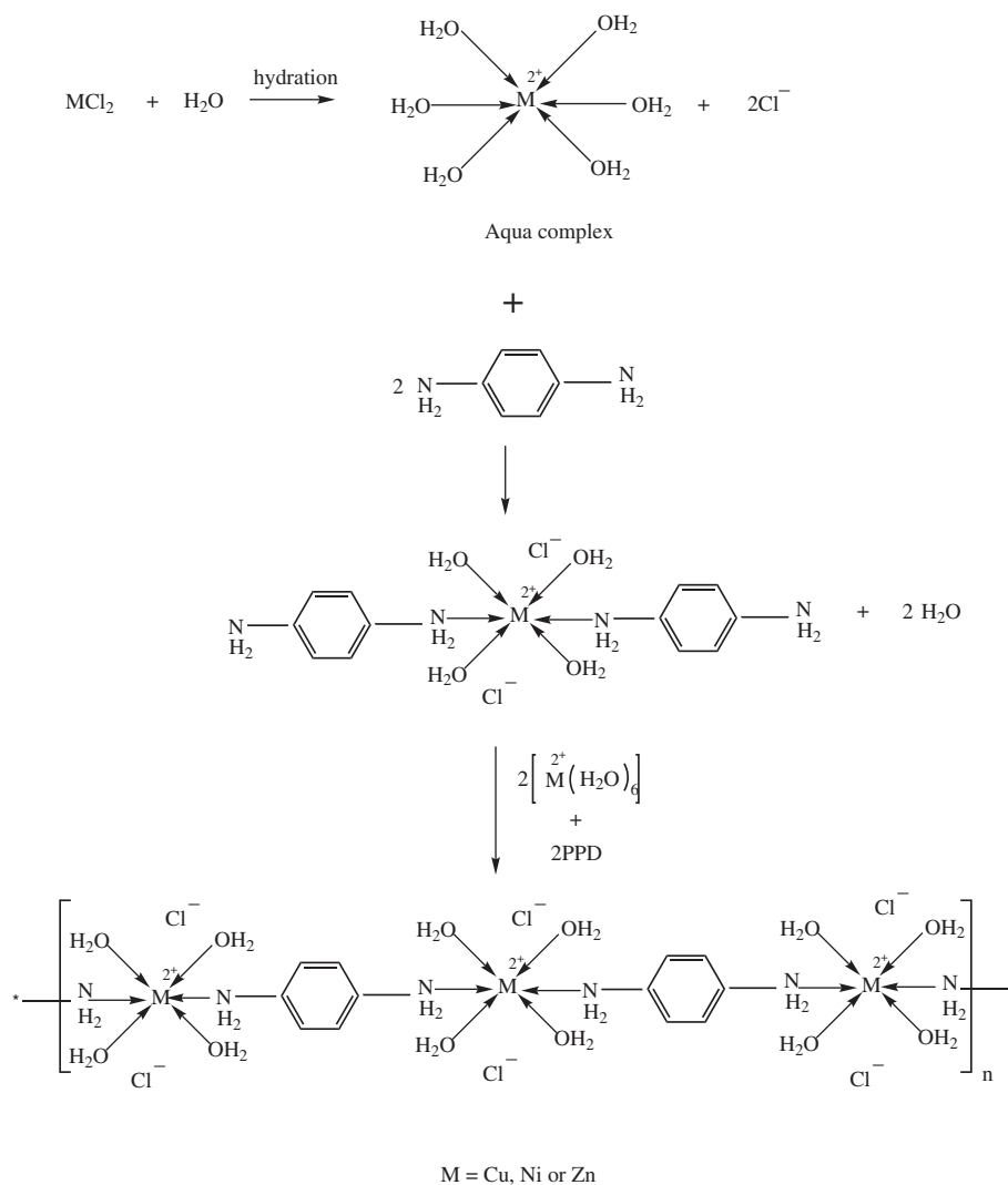
Scheme 2 Proposed mechanism.
