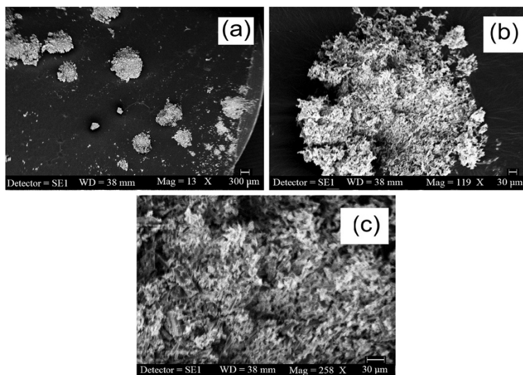
Figure 9 Typical SEM images of the particles of 3 . (a) Low magnification SEM image, (b) and (c) high magnification SEM images.
