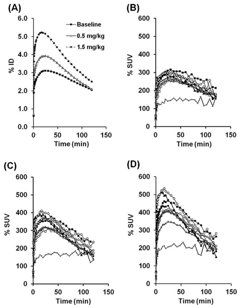
Figure 5 Time-activity curves of brain radioactivity after intravenous injection of [ ^{11}\text{C} ]N-methyl-SSR504734 in a cynomolgus monkey. At baseline and pretreatment conditions (0.5 or 1.5 mg/kg of SSR504734). Whole brain uptake was expressed as percent injected dose (%ID) (A). Regional brain uptake was expressed as percent standard uptake value (%SUV) under baseline (B), pretreatment of SSR504734 (0.5 mg/kg) (C), and pretreatment of SSR504734 (1.5 mg/kg) conditions (D). Black square, thalamus; white circle, pons; black triangle, cerebellum; white diamond, putamen; asterisk, frontal cortex; cross, white matter; black circle, caudate; white square, anterior cingulate cortex; white triangle, temporal cortex.
