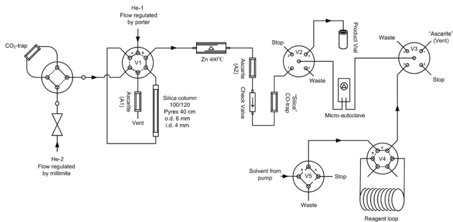
Figure 1 Schematic overview of the synthesis unit used to synthesize [ 11 C]CO.
