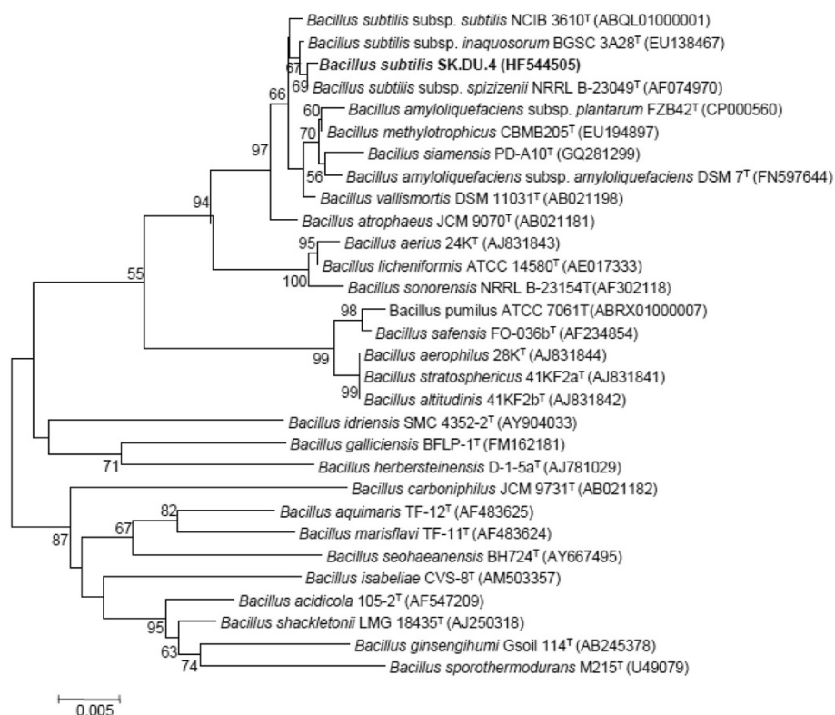
Figure 1 Neighbour-joining phylogenetic tree based on 16S rRNA gene sequences, showing the phylogenetic relationship between strain SK.DU.4 and other members of the genus Bacillus . Bootstrap values greater than 50% are given at the nodes.
