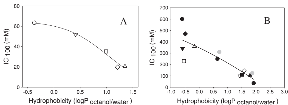
Figure 2 Hydrophobicity as \log P_{\text{octanol/water}} partition coefficients plotted with the minimal inhibitory concentrations ( IC_{100} ) of aldehydes. A) HMF ( \circ ), furfural ( \nabla ), syringaldehyde ( \square ), vanillin ( \diamond ), and 4-hydroxybenzaldehyde ( \Delta ); and organic acid compounds B) ammonium lactate ( \bullet ), ammonium levulinate ( \blacklozenge ), ammonium succinate ( \blacktriangledown ), ammonium formate ( \square ), ammonium acetate ( \Delta ), ammonium 2-furoate ( \circ ), ammonium itaconate (gray octagon), ammonium vanillate ( \nabla ), ammonium ferulate ( \blacksquare ), ammonium 4-hydroxybenzoate ( \diamond ), ammonium 4-hydroxycinnamate ( \blacktriangle ), ammonium benzoate (gray hexagon), and ammonium caproate ( \bullet ).
