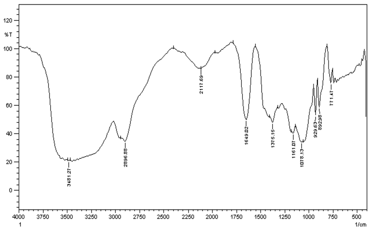
Figure 3 FTIR spectrum of agarose.
