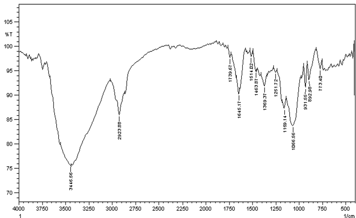
Figure 4 FTIR spectrum of MB-adsorbed agarose.
