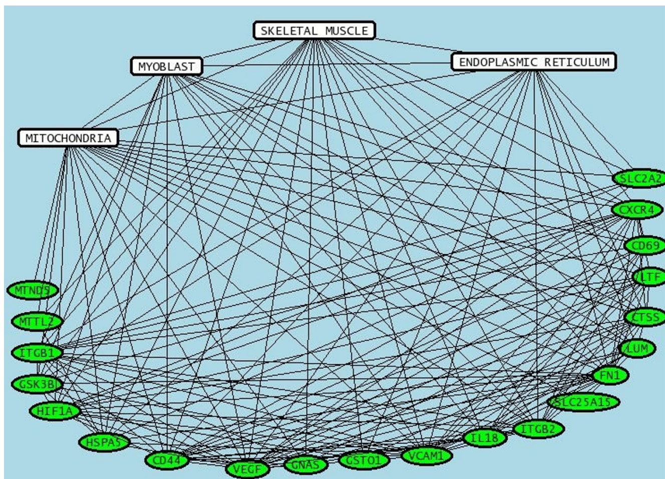
Figure 4 Relationships between pairs of genes and cellular compartments. The analysis of the main metabolic pathways and their dysfunctions was performed using a data mining software (Predictsearch®). Briefly, gene aliases corresponding to the significant modulated genes were submitted as queries to PubMed in order to collect titles and abstracts of all related publications. The results showed that a part of the significant modulated genes were strongly associated with the following terms: skeletal muscle, mitochondria, myoblast, endoplasmic reticulum.
