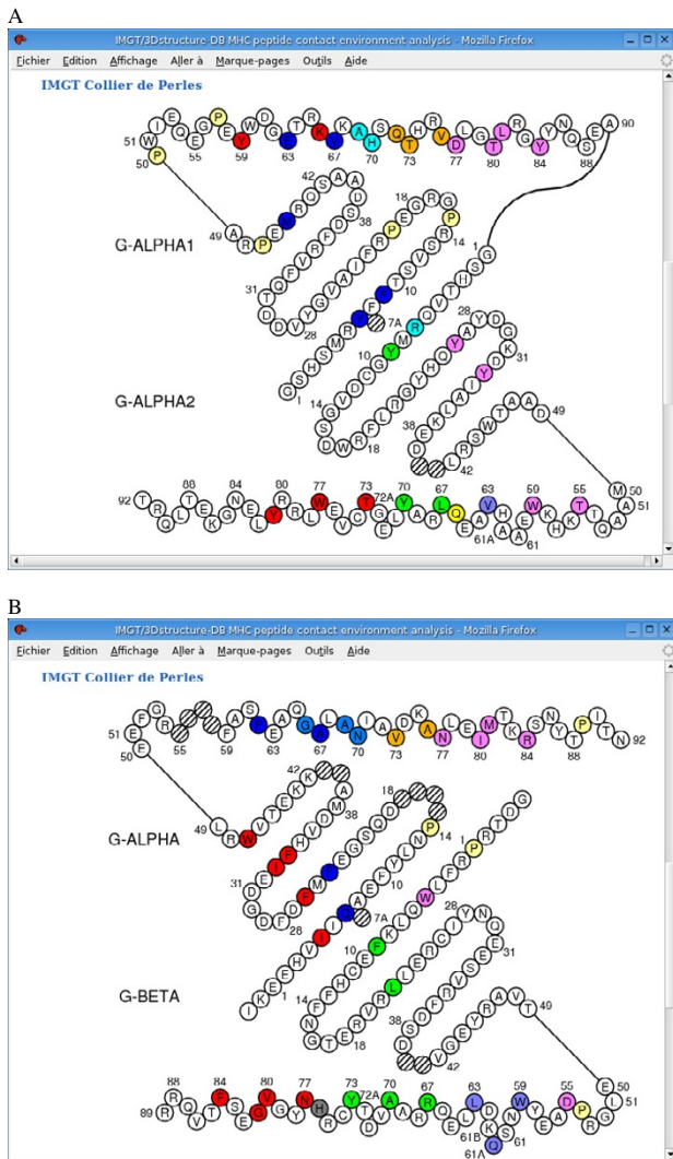
Figure 3 IMGT Colliers de Perles of the two G-DOMAINS of MHC class I (A) and of MHC class II (B) proteins (codes PDB 1bd2 and 1aqd, respectively, in IMGT/3Dstructure-DB [9]). The IMGT Collier de Perles of a G-DOMAIN is based on the IMGT unique numbering for G-DOMAIN and G-LIKE-DOMAIN [18]. (A) The two MHC-I G-DOMAINS, G-ALPHA1 (top) and G-ALPHA2 (bottom), form the groove of the MHC class I chain (I-ALPHA). (B) The two MHC-II G-DOMAINS, G-ALPHA (top) of the MHC class II alpha chain (II-ALPHA) and G-BETA (bottom) of the MHC class II beta chain (II-BETA), form the groove of the MHC class II protein [36]. Amino acids are shown in the one-letter abbreviation. Hatched circles correspond to missing positions according to the IMGT unique numbering [18]. Positions in colour correspond to the IMGT contact sites provided, for each peptide/MHC 3D structure, in IMGT/3Dstructure-DB [36].
